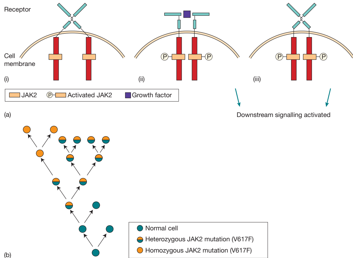
Figure 15.2 The role of JAK2 mutation in the generation of myeloproliferative diseases. (a) (i) Most haemopoietic growth factor receptors do not have intrinsic kinase activity but associate with a protein kinase such as JAK2 in the cytoplasm. (ii) When the receptor binds a growth factor (e.g. erythropoietin) the cytoplasmic domains move closer together and the JAK2 molecules can activate each other by phosphorylation and phosphorylate downstream proteins e.g. STATS (Fig. 1.7). (iii) The V617F JAK2 mutation allows the JAK protein to become activated even when no growth factor is bound. (b) A model for the development of myeloproliferative disease following JAK2 mutation. The primary event appears to predispose to an acquired heterozygous mutation of JAK2 (V617F). This leads to a survival advantage. In some patients, a mitotic recombination event leads to a homozygous JAK2 mutation state.
