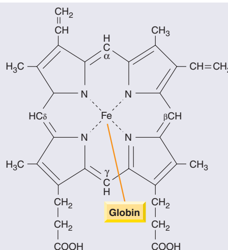
Figure 2.8 The structure of haem.
